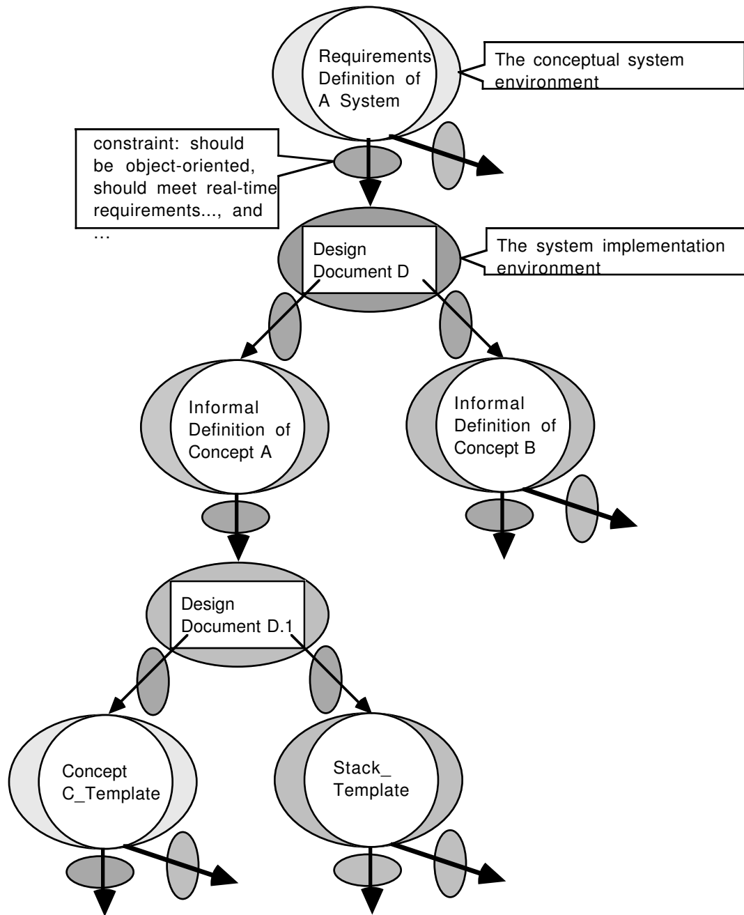
Figure 4 — A Structure of Life cycle Assets of A Software System
