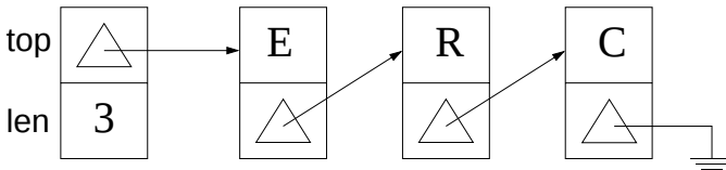
Fig. 2. Representation of a Stack \langle \text{char} \rangle with abstract value \langle E, R, C \rangle
