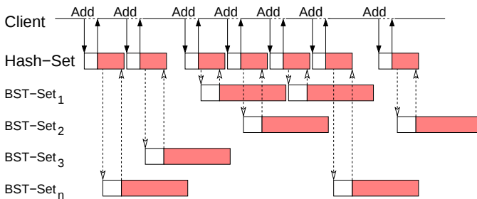
Fig. 13. Execution of \text{ER-Set} = \text{Hash-Set} \langle \text{BST-Set} \rangle
