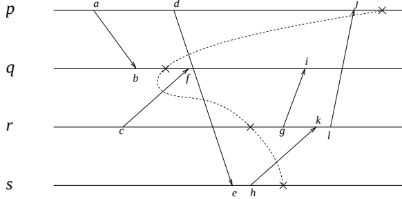
Figure 2. An inconsistent cut in a distributed system
