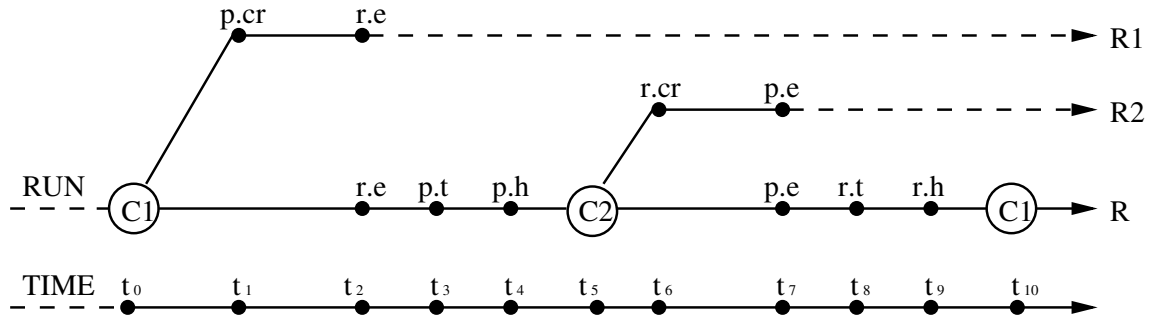
Figure 6. Any partial run up to C_1 can be extended to re-visit C_1 before q eats.
