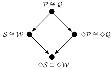
Figure 4. The Chandra-Toueg hierarchy consists of four equivalence classes of failure detectors. Failure detector classes higher in the lattice are strictly stronger than detector classes lower in the lattice.
